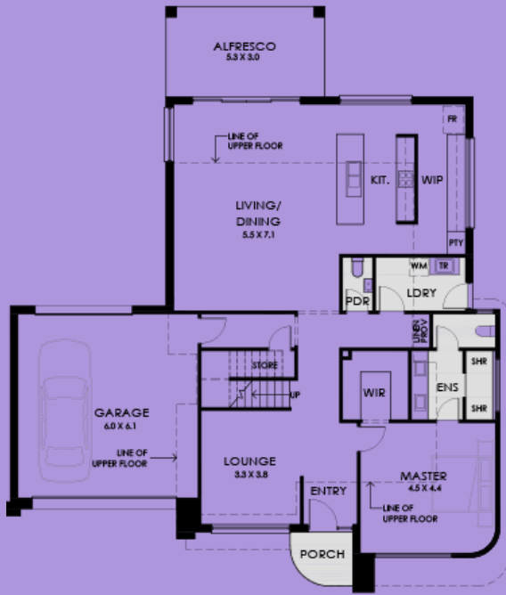
GROUND LEVEL
